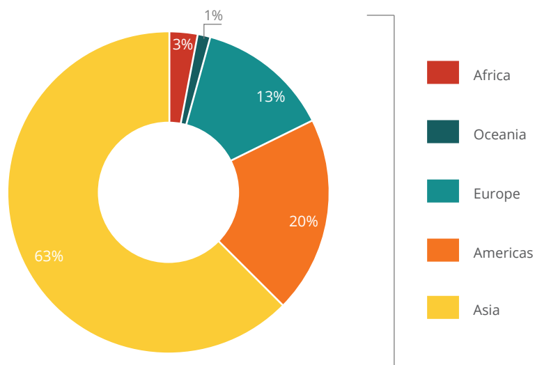
FIGURE 4-10a Synthetic fertilizers, 2001-2011: emissions by continent.
