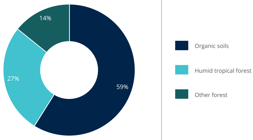
FIGURE 5-9 Burning biomass by sub-sector, 2001-2011.
